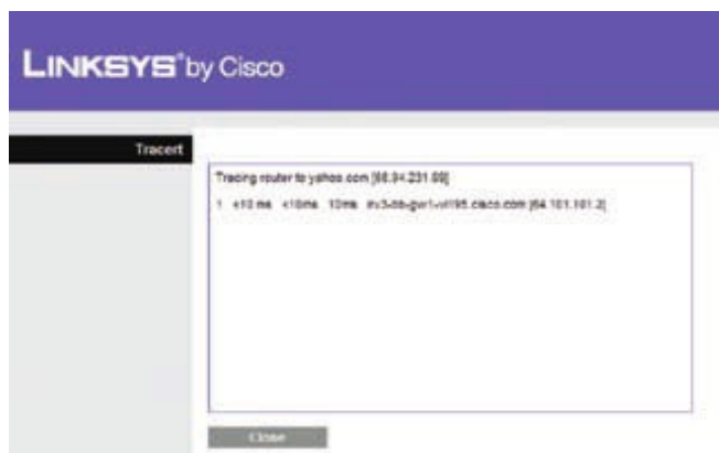
Traceroute Test
